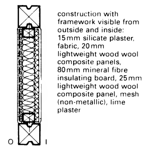
9 New panel
